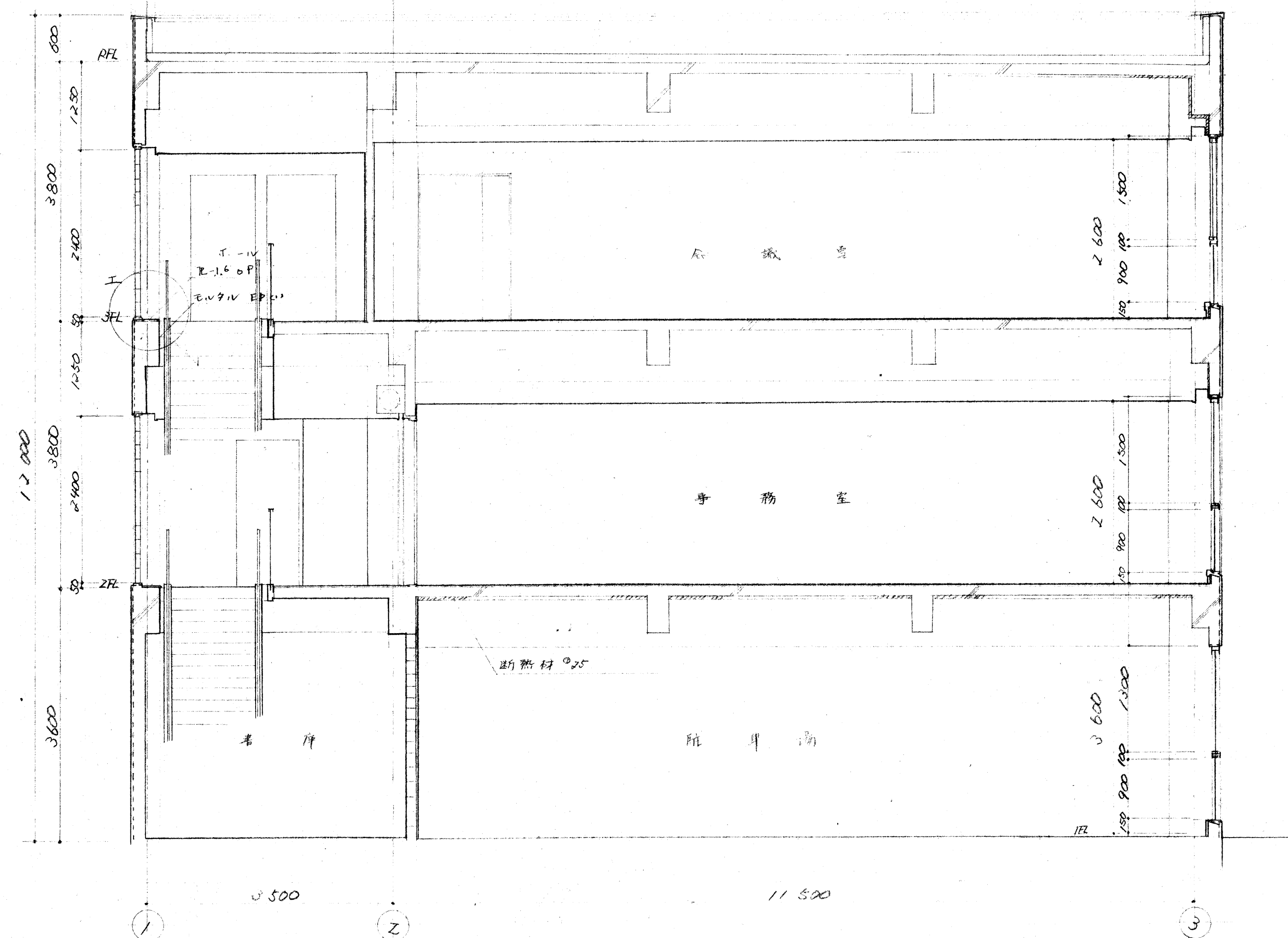
×-× 矩. 荷 固 S_1 = 50
